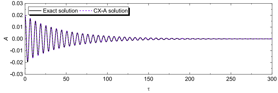
(a) Displacement of primary structure
