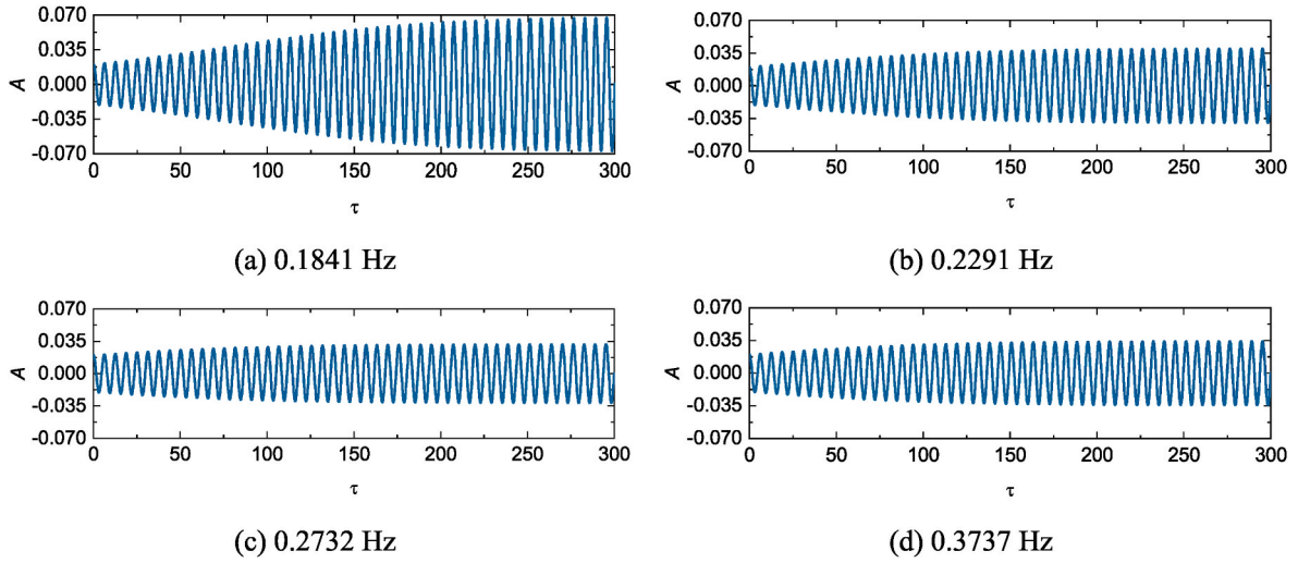
Fig. 21. VIVs of long-span bridge without control.
