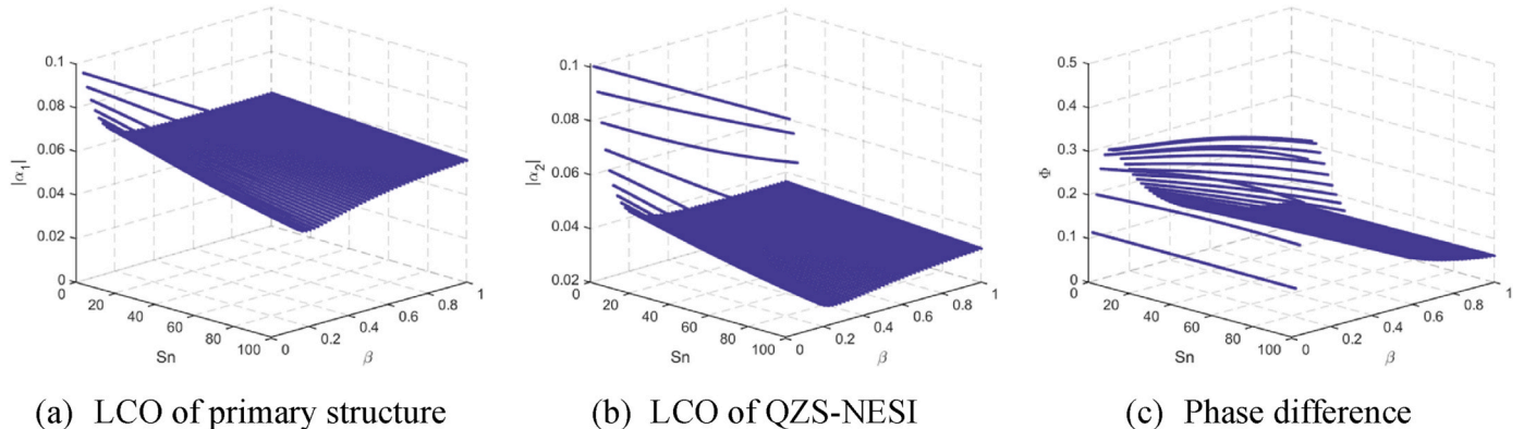
Fig. 15. Bifurcation diagram of system with respect to cubic stiffness S_n and inertance ratio \beta
