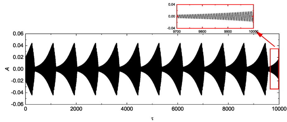
(c) SMR with S_n = 50 and \eta_1 = 0.01
