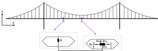
Fig. 2. Long-span bridge with QZS-NESI system.
