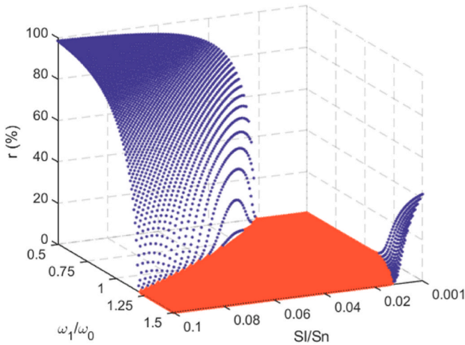
Fig. 27. VIV reduction ratio versus \omega_1/\omega_0 and S_l/S_n .
