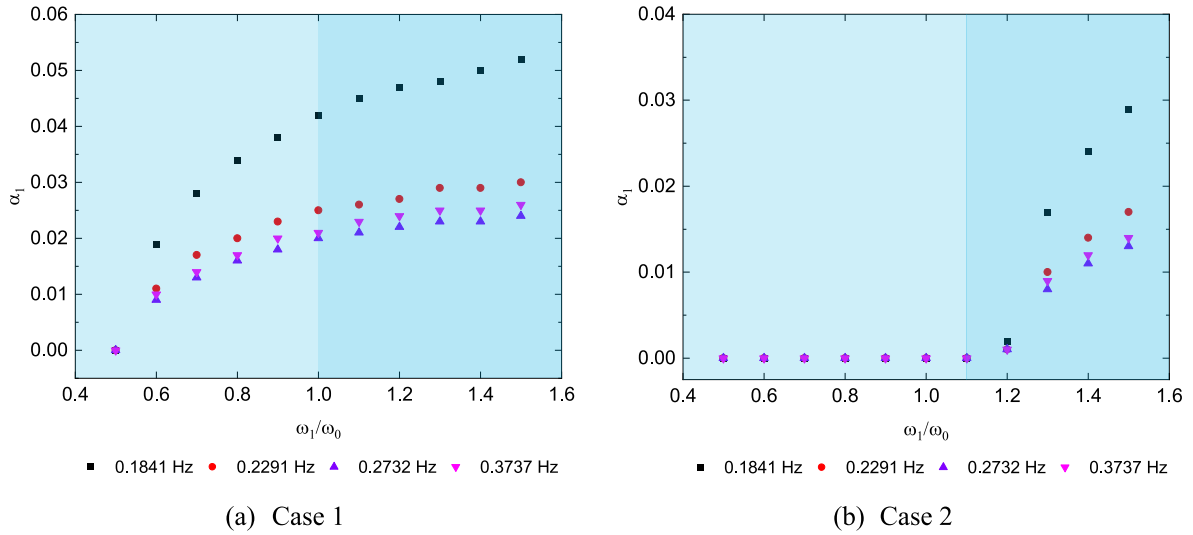
Fig. 25. VIV amplitudes under variations at each structural frequency.
