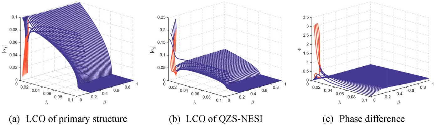
Fig. 16. Bifurcation diagram of system with respect to mechanical damping \lambda and inertia ratio \beta
