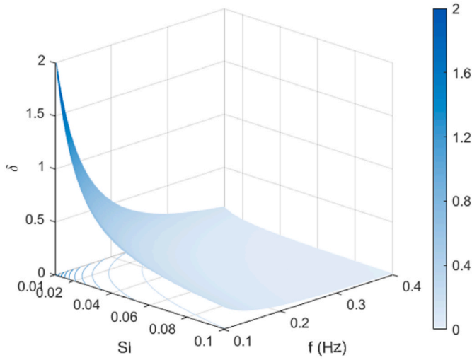
Fig. 26. Static stroke versus S_l and modal frequency ( \mu = 0.001 , \beta = 0.4 , and \alpha = 1/200 ).
