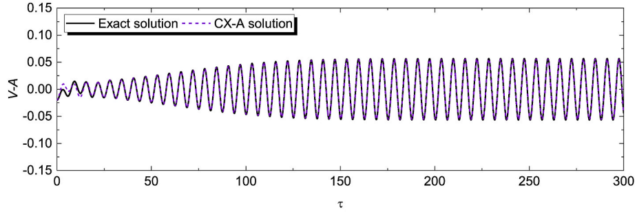
(b) Displacement of QZS-NESI
