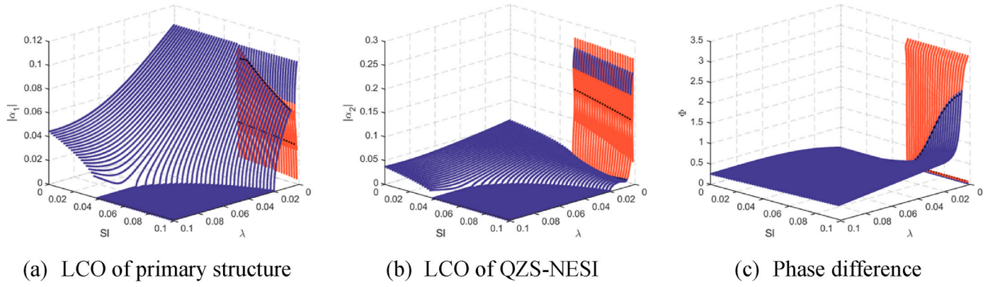
Fig. 11. Bifurcation diagram of system with respect to mechanical damping \lambda and linear stiffness S_l
