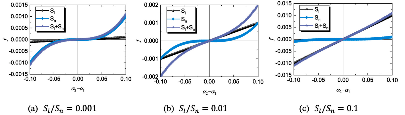
Fig. 12. Dimensionless restoring force versus relative displacement with different stiffness ratios.
