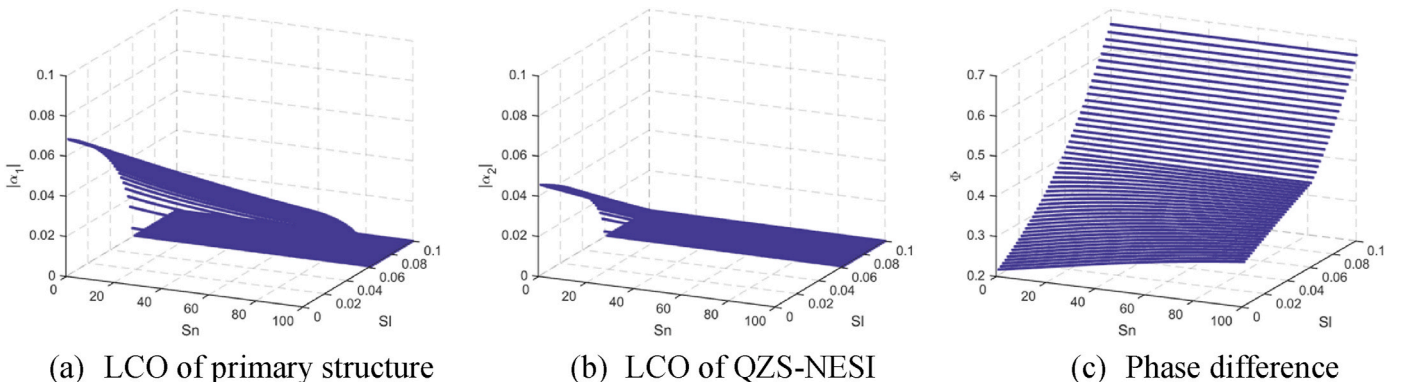
Fig. 10. Bifurcation diagram of system with respect to cubic stiffness S_n and linear stiffness S_l
