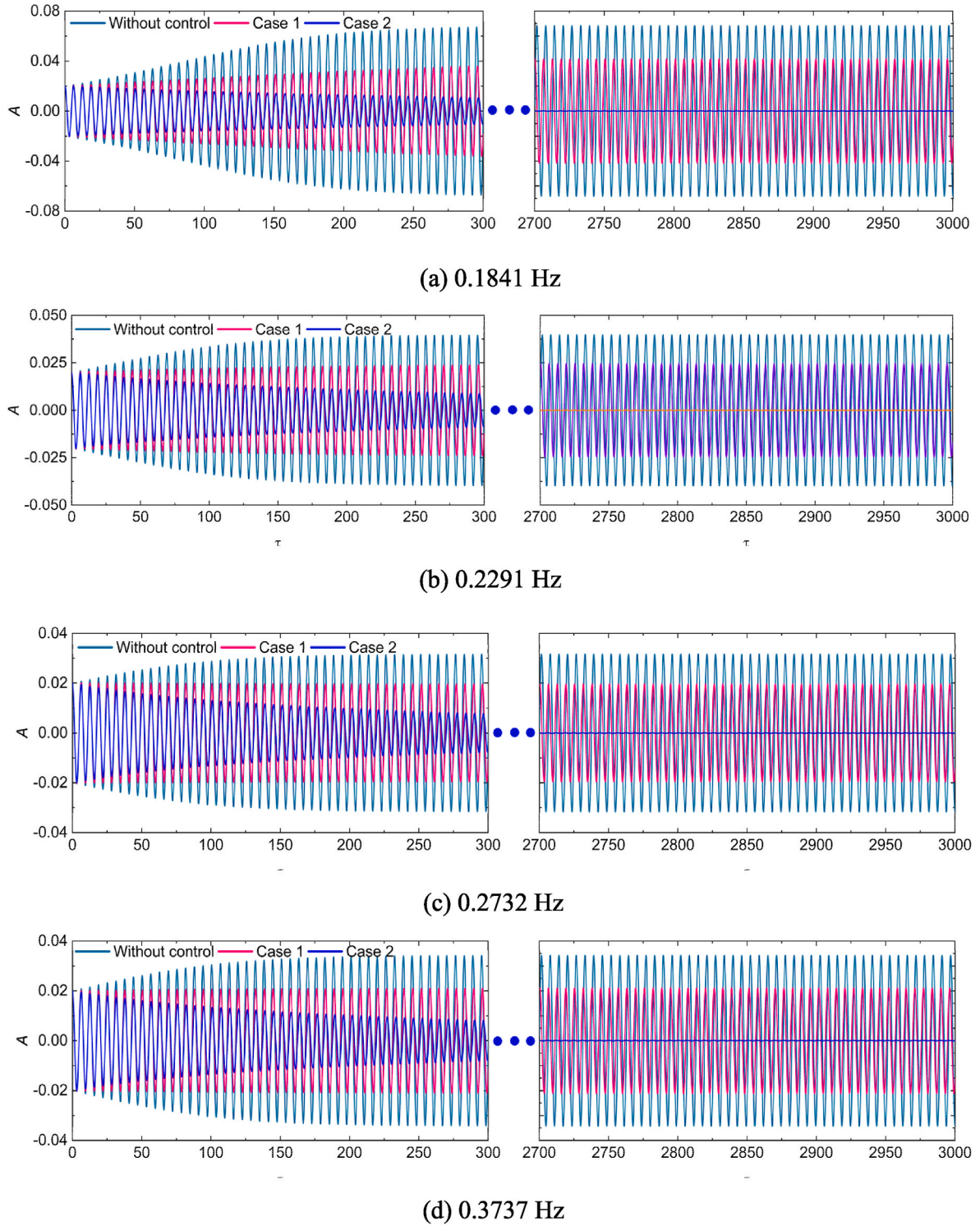
Fig. 23. VIVs of long-span bridge with QZS-NESI.
