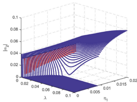
(b) LCO of QZS-NESI
