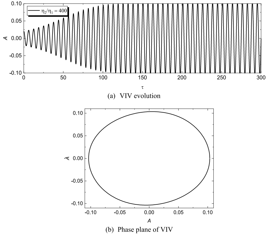
Fig. 6. VIV of beam with aerodynamic parameters of \eta_2/\eta_1 = 400 .
