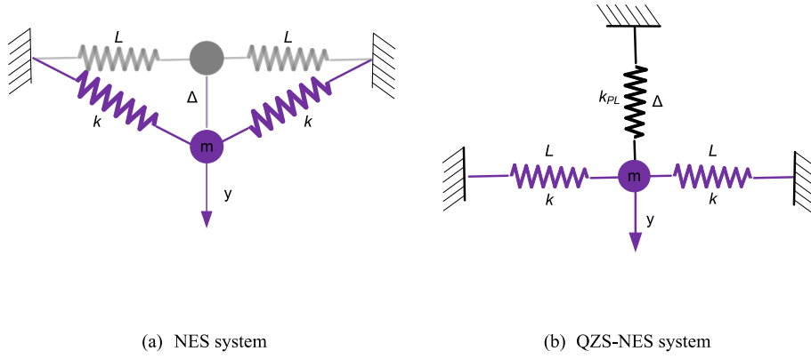
Fig. 1. Vertical static equilibrium state under weight.
