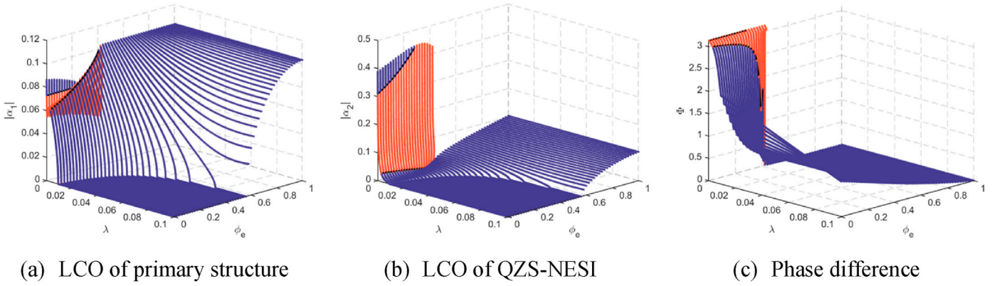
Fig. 18. Bifurcation diagram of system with respect to mechanical damping \lambda and modal value \phi_e
