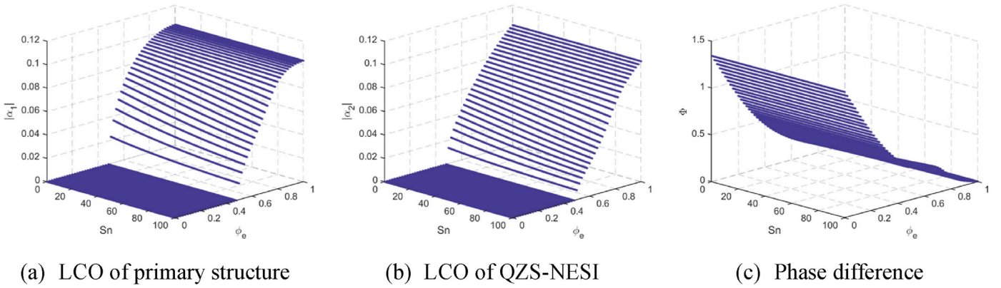
Fig. 17. Bifurcation diagram of system with respect to cubic stiffness S_n and modal value \phi_e
