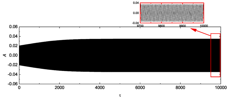
(b) Suppressed LCO with S_n = 50 and \eta_1 = 0.003
