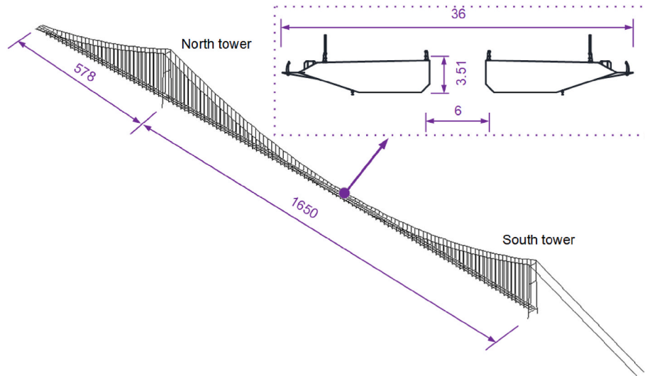
Fig. 19. Layout of Xihoumen Bridge (unit: m).
