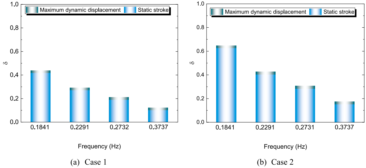
Fig. 24. Displacement of QZS-NESI under VIVs ( \alpha = 1/200 for conservative consideration).
