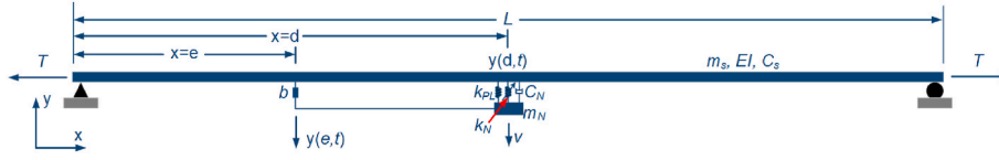
Fig. 3. Tensioned beam with QZS-NESI system.
