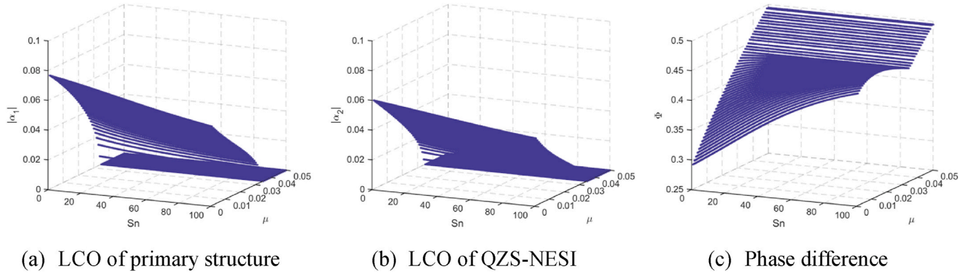
Fig. 13. Bifurcation diagram of system with respect to cubic stiffness S_n and mass ratio \mu
