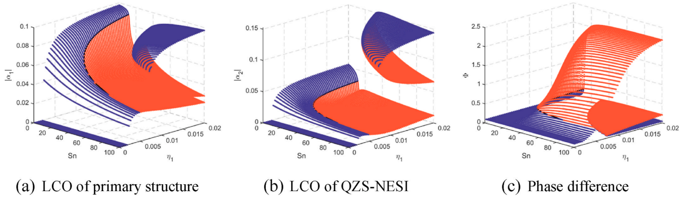
Fig. 7. Bifurcation diagram of system with respect to cubic stiffness S_n and aerodynamic parameter \eta_1
