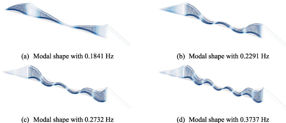
Fig. 20. Modal shapes of Xihoumen Bridge corresponding to VIV occurrence.
