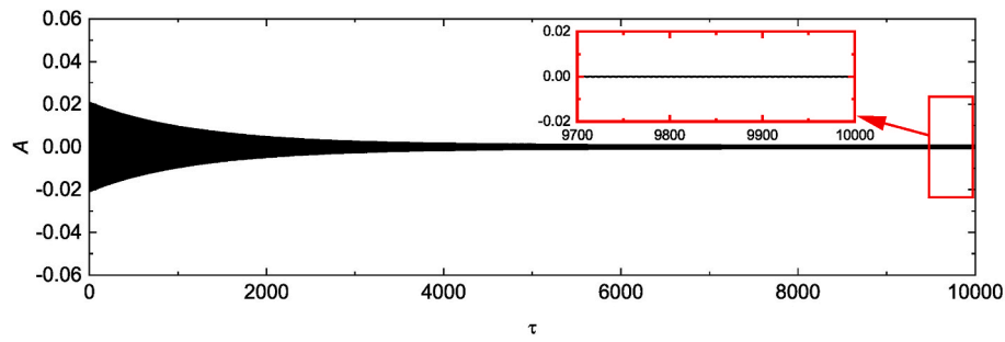
(a) Eliminated LCO with S_n = 50 and \eta_1 = 0.0005
