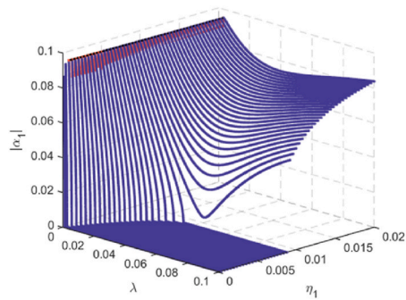
(a) LCO of primary structure
