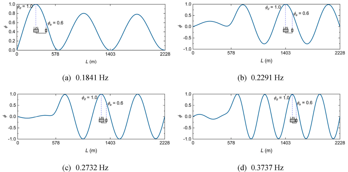
Fig. 22. Normalized mode shapes and NESI installation configuration.
